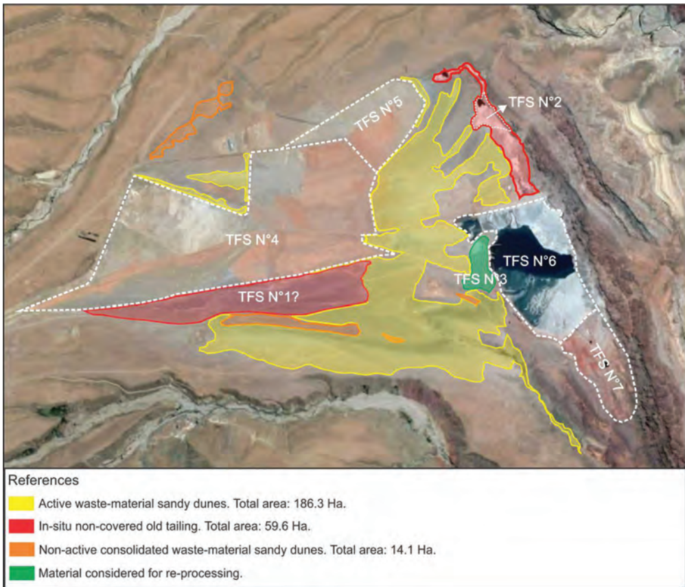
Figure 1 Main lithotypes for wind-remobilized tailings.
