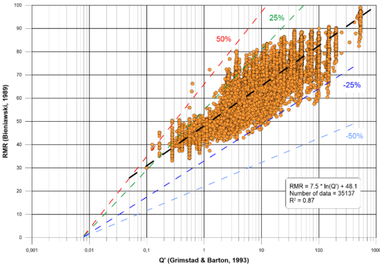
Figure 3. Bieniawki RMR [2] vs. Q System [3] correlation.
